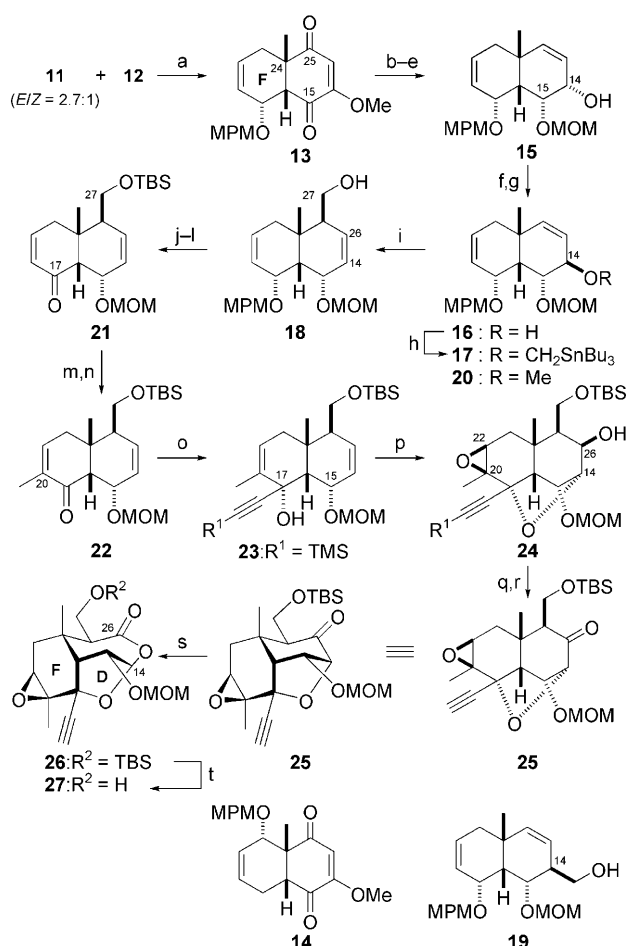
Scheme 3. Synthesis of seven-membered lactones 26 and 27 . Reagents and conditions: a) toluene, 100°C, 3 days, ( 13 , 63%; 14 , 19%); b) DIBAL-H, \text{CH}_2\text{Cl}_2 , 0°C; c) 10% aq \text{H}_2\text{SO}_4 , \text{CH}_2\text{Cl}_2 , RT (74%, over 2 steps); d) MOMCl, i\text{Pr}_2\text{NEt} , \text{CH}_2\text{Cl}_2 , reflux (98%); e) \text{NaBH}_4 , \text{CeCl}_3 \cdot 7\text{H}_2\text{O} , MeOH, RT (98%); f) DIAD, \text{PPh}_3 , p\text{NO}_2\text{PhCOOH} , THF, RT; g) \text{K}_2\text{CO}_3 , MeOH/ \text{Et}_2\text{O} (3:1), RT (86%, over 2 steps); h) \text{Bu}_3\text{SnCH}_2\text{I} , NaH, DMF/THF (1:1), RT (76%); i) MeLi in \text{Et}_2\text{O} , THF, 0°C ( 18 , 72%; 19 , 9%; 16 , 10%; yields were determined by ^1\text{H} NMR spectroscopy; 20 , 5%); j) TBSCl, \text{Et}_3\text{N} , DMAP, \text{CH}_2\text{Cl}_2 , RT; k) DDQ, \text{CH}_2\text{Cl}_2 , pH 7 buffer, RT (68%, over 3 steps from 17 ); l) \text{MnO}_2 , \text{CH}_2\text{Cl}_2 , RT (93%); m) \text{TMSN}_3 ; then \text{I}_2 , pyridine, \text{CH}_2\text{Cl}_2 , 0°C to RT; n) \text{MeMgBr} , \text{Fe}(\text{acac})_3 , NMP, THF, 0°C (73%, over 2 steps); o) TMS-acetylene, n\text{BuLi} , \text{CeCl}_3 , THF, -78^\circ\text{C} (96%); p) m CPBA (10 equiv), \text{CH}_2\text{Cl}_2 , 0°C to RT (73%); q) \text{K}_2\text{CO}_3 , MeOH; r) Dess–Martin periodinane, \text{CH}_2\text{Cl}_2 , RT (92%, over 2 steps); s) m CPBA, \text{NaHCO}_3 , \text{CH}_2\text{Cl}_2 , RT (92%); t) HF-pyridine, \text{CH}_2\text{Cl}_2 /pyridine (1:1), 0°C (93%). acac = acetylacetonate, Bu = butyl, DDQ = 2,3-dichloro-5,6-dicyano-1,4-benzoquinone, DIAD = diisopropylazodicarboxylate, DIBAL-H = diisobutylaluminum hydride, DMAP = 4-dimethylaminopyridine, DMF = N,N -dimethylformamide, m CPBA = meta -chloroperoxybenzoic acid, MOM = methoxymethyl, NMP = N -methylpyrrolidone, TBS = tert -butyldimethylsilyl, THF = tetrahydrofuran, TMS = trimethylsilyl.
