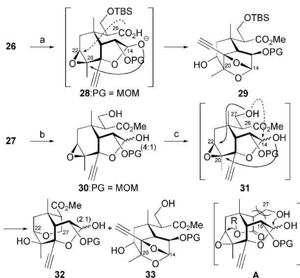
Scheme 4. Attempts at the formation of the G ring or H ring. Reagents and conditions: a) LiOH·H 2 O, THF/H 2 O (1:1), RT; then TMSCHN 2 , Et 2 O/MeOH (86%); b) LiOH·H 2 O, MeOH, 0 °C; c) CSA, CH 2 Cl 2 , RT ( 32 , 56%; 33 , 10% over 2 steps). CSA = (±)-camphorsulfonic acid.
